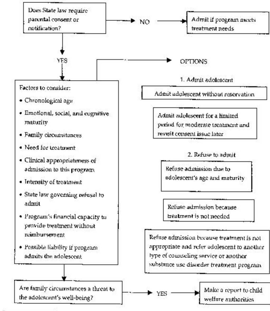
Figure 8-1: Decision Tree
